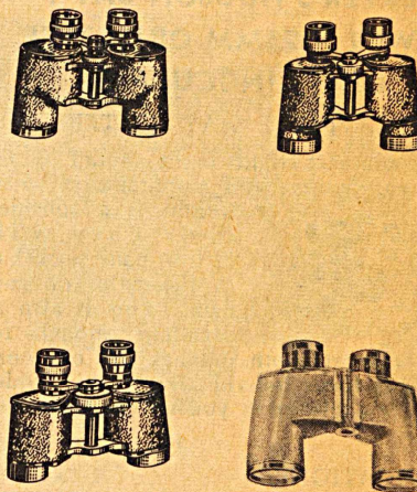
Figure 1—American Mon-a-block construction. Figure 2—German two-piece construction. Figure 3—French box construction. Figure 4—California style outside body using mon-a-block construction.
