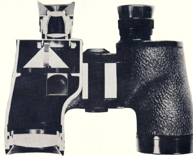
Cross section of our Precision Binoculars showing how prisms are set on metal shelf and firmly held into position with metal bands.
