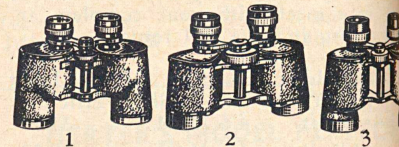
Figure 1—Bausch & Lomb originated Mon-a-block. Used by Herter's. Figure 2—Obsolete German two-piece construction. Figure 3—Very obsolete French box construction.
