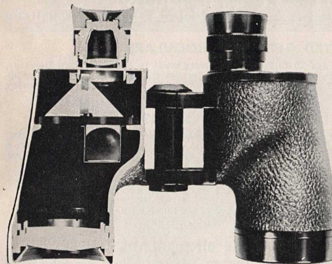
Cross section of our Precision Binoculars showing how prisms are set on metal shelf and firmly held into position with metal bands.
