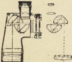
Construction of 7 x 50
