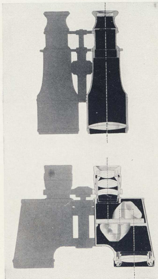
Top: Galilean Field Glass. Bottom: Bausch & Lomb Prism Binocular.
