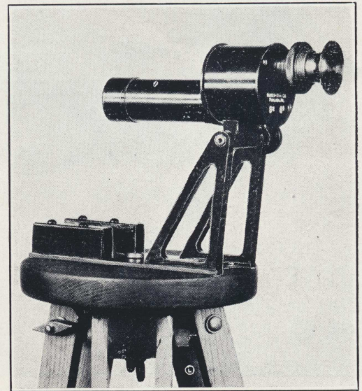
PELORUS PRISMATIC TELESCOPE
