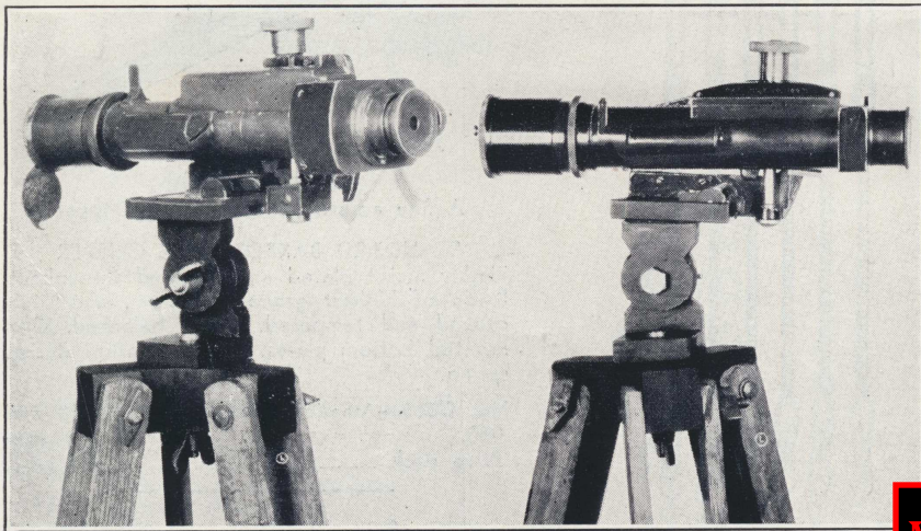
U. S. ARMY PRISMATIC GUN SIGHTS
